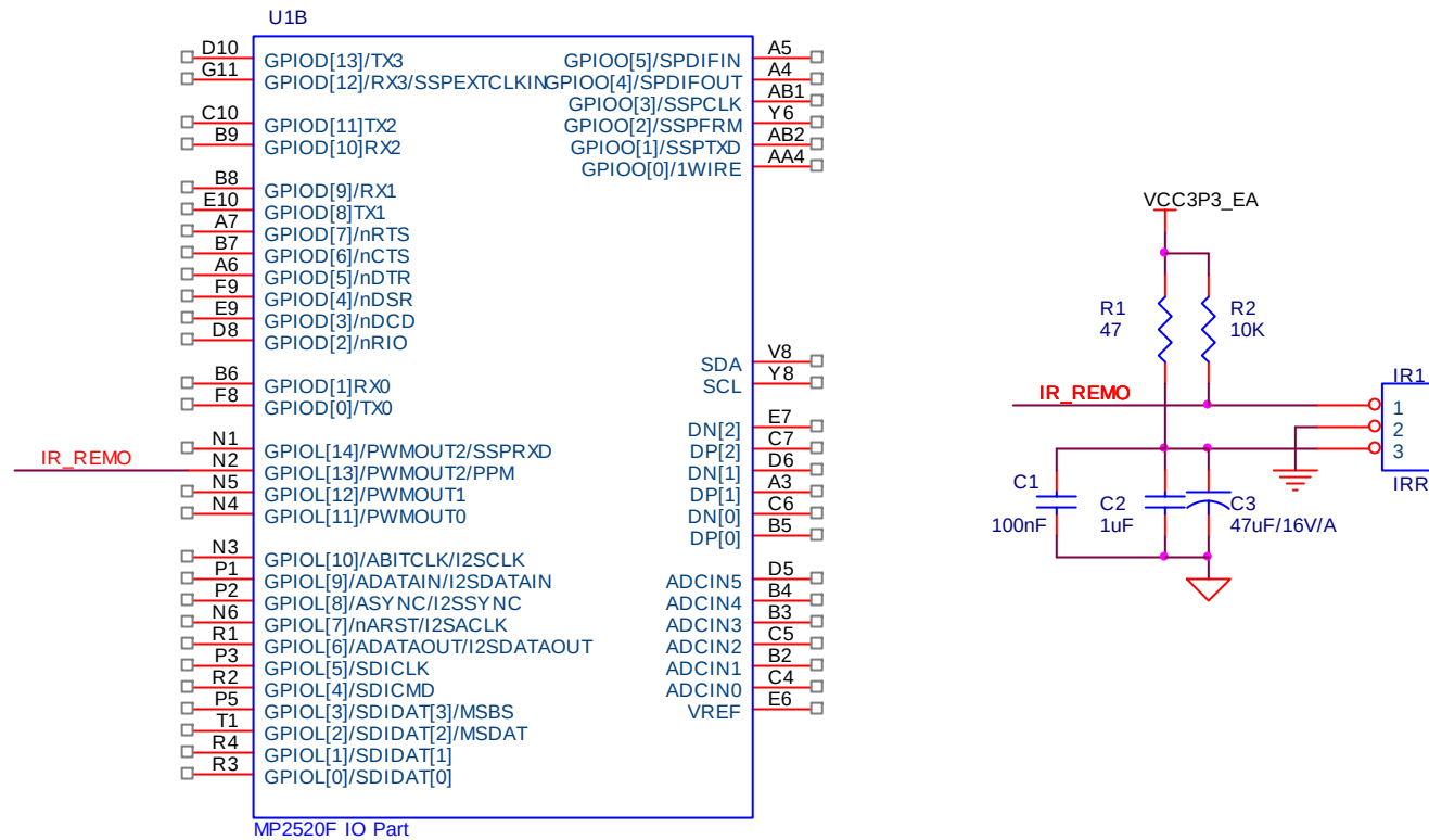
<Figure 12-1. Design guide of PPM>
