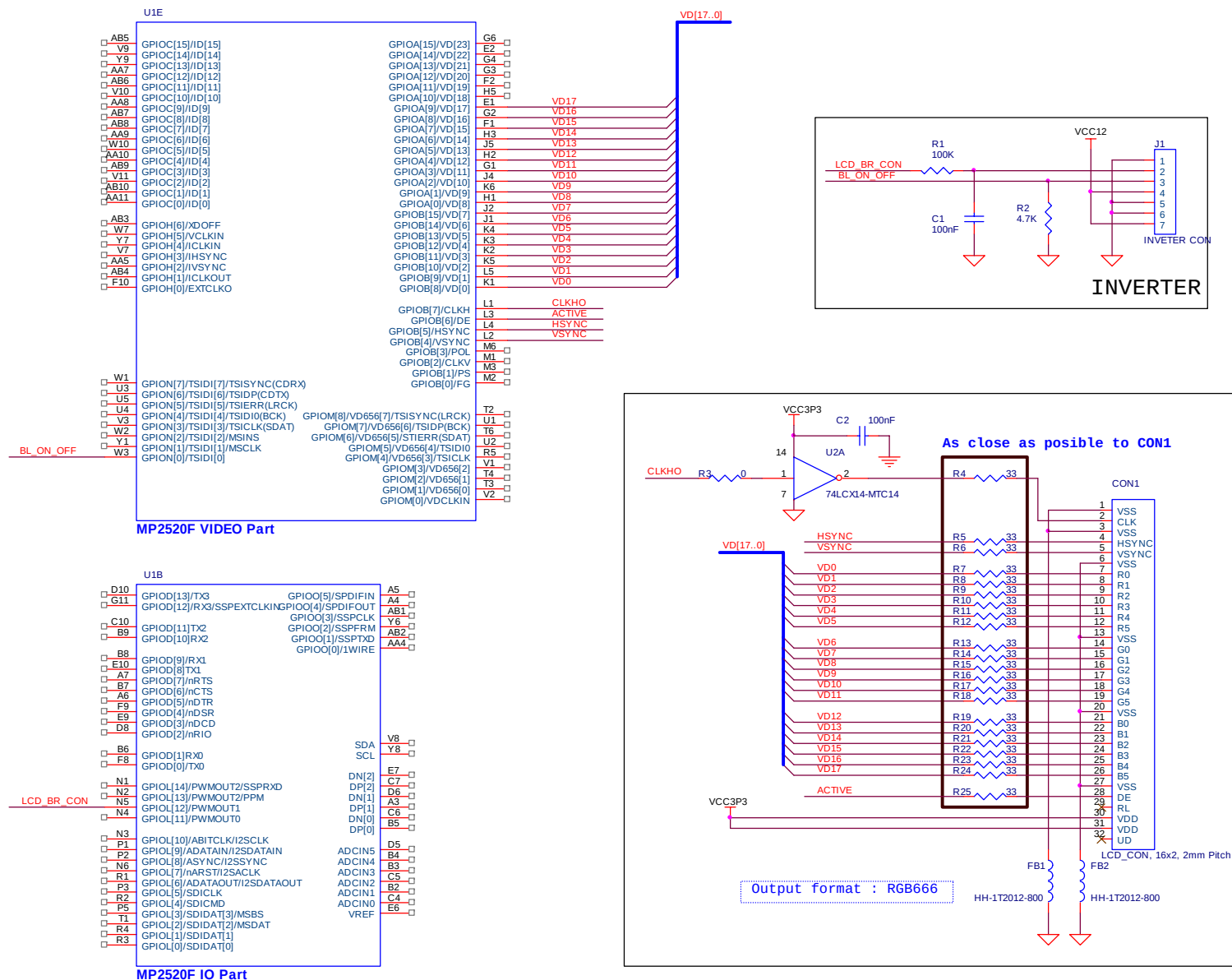
<Figure 7-1. Design guide of LCD Module interface>
